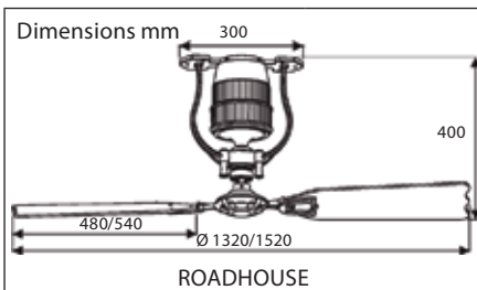
ROADHOUSE MA #413280 housing antique brass, here with 4 blades an- tique oak (see picture)/walnut #19601 , Ø132 cm
